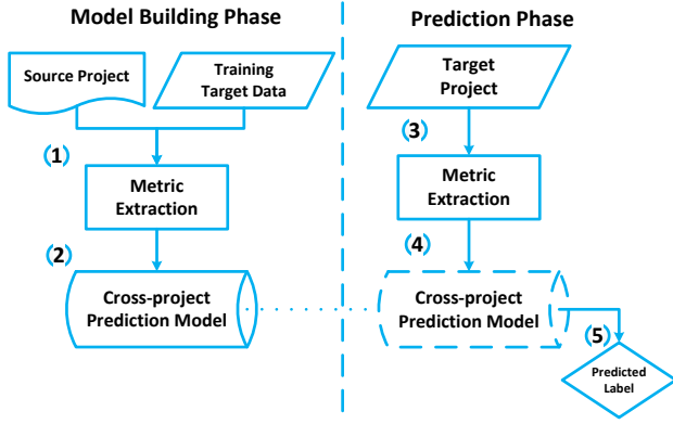
Fig. 1. Overall architecture of CroBuild .
