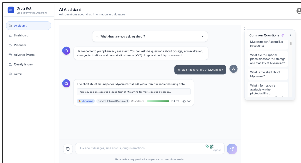
Figure 2: User Interface of the Pharmaceutical Chatbot. The UI shows the questions asked by the user, the response by the chatbot, the identified drug in the question, the source of the information used for the answer and the confidence score for the response.
